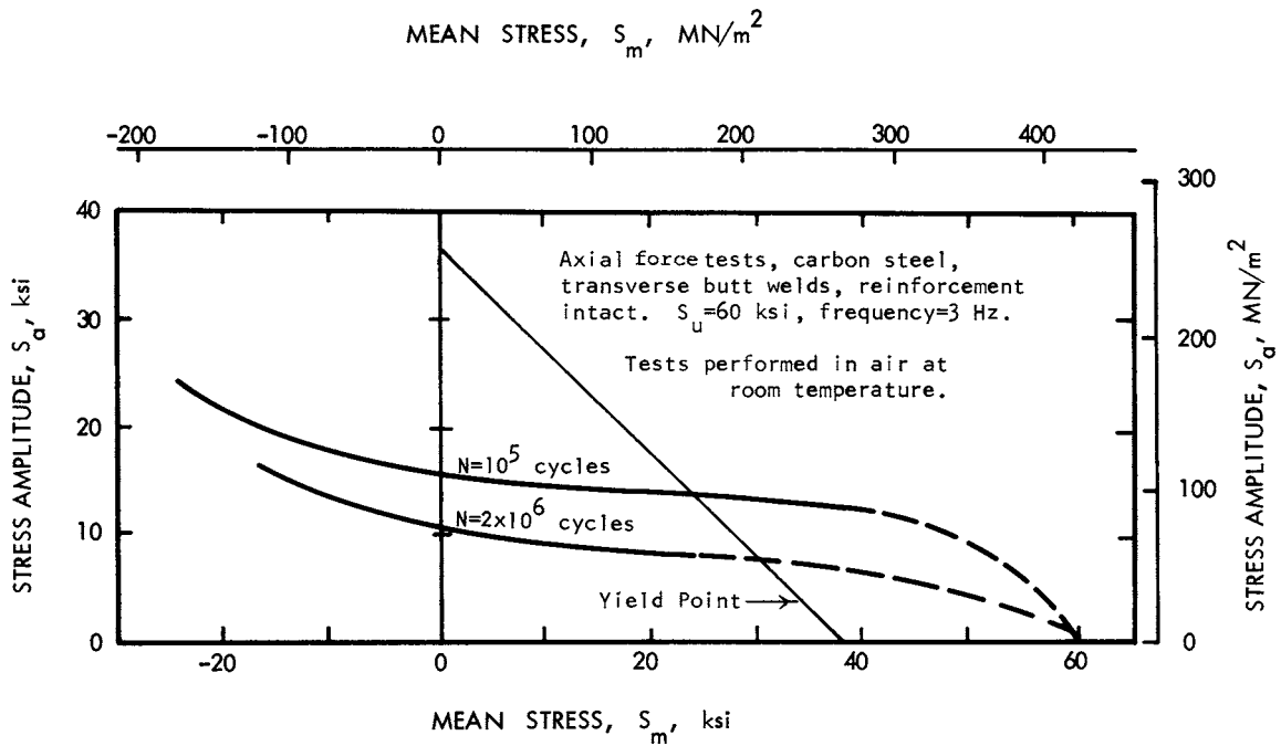
FIG. 3 Constant-Life Diagram
