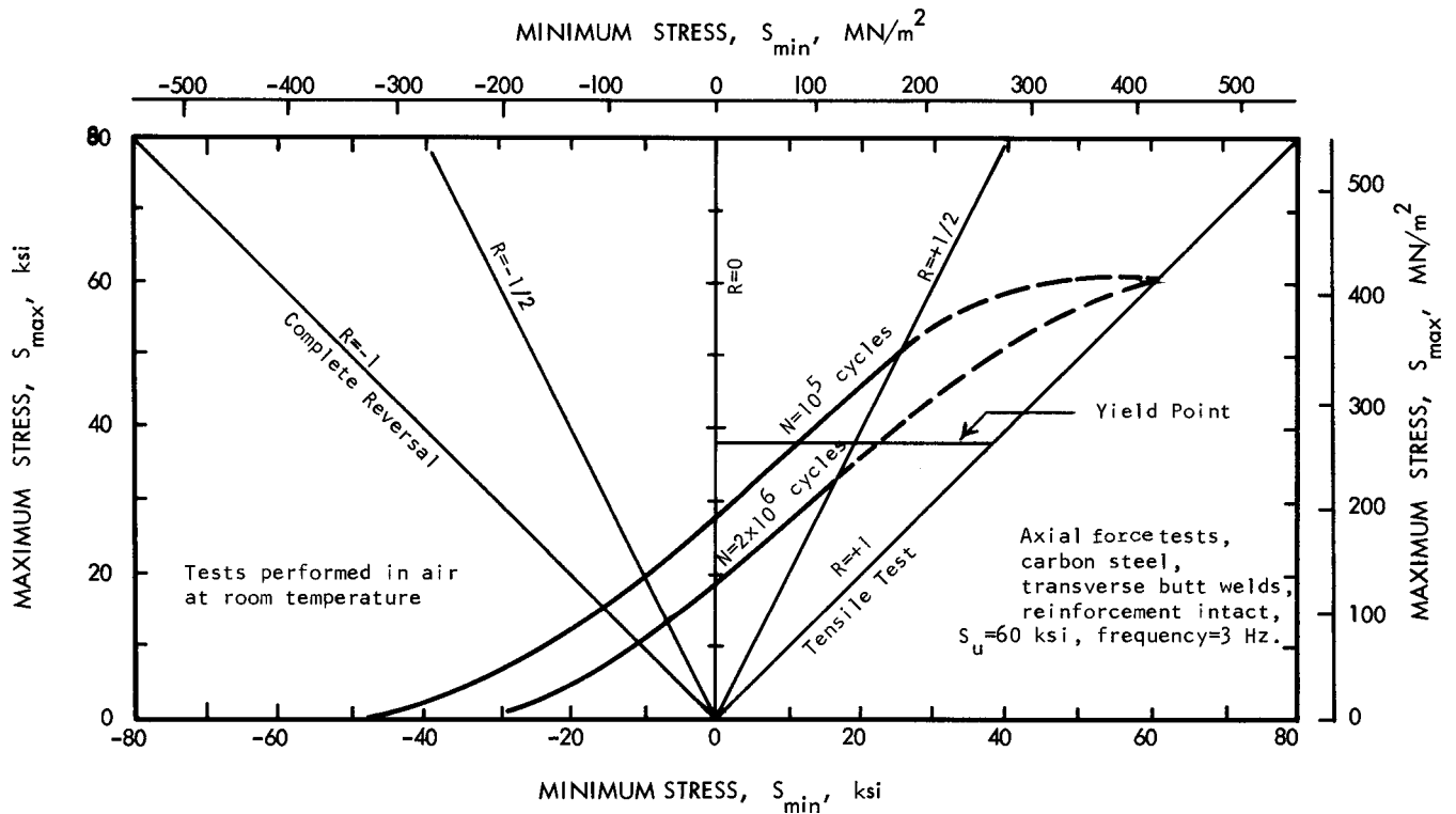
FIG. 2 Constant-Life Diagram
