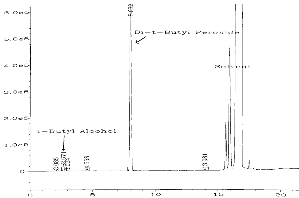
FIG. 1 Typical Chromatogram
