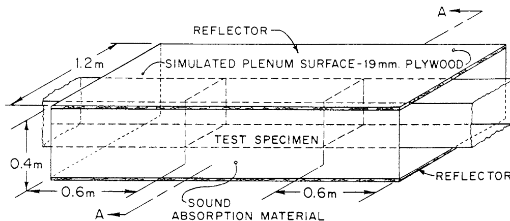
FIG. 5 Simulated Semi-Reflective Plenum Configuration
