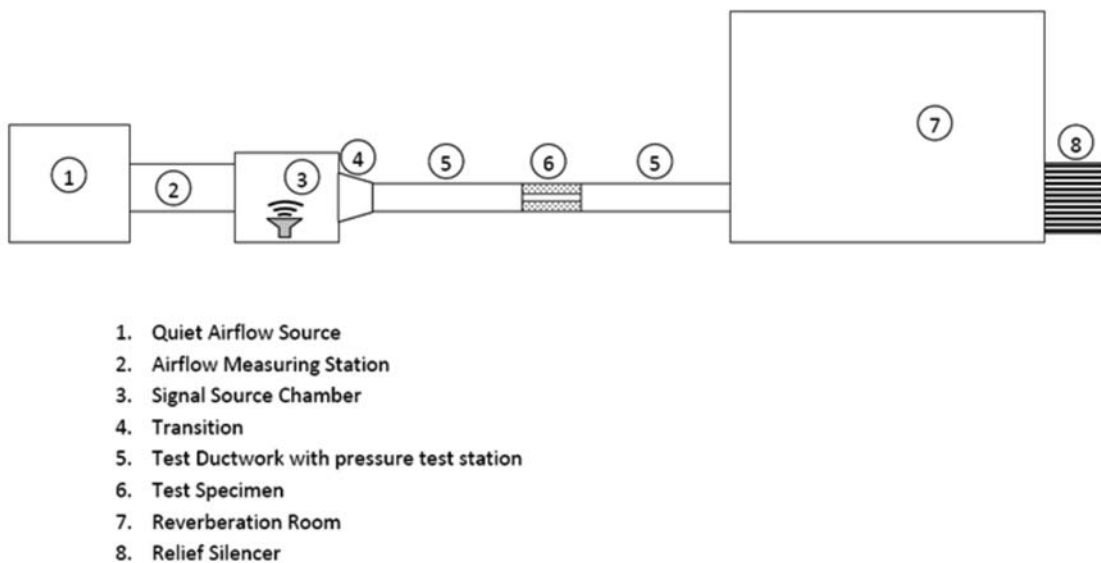
FIG. 1 Typical Facility for Rating Straight Duct Silencers With or Without Airflow
