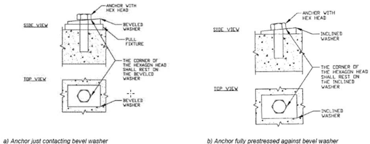
FIG. 14 Acceptable Position of the Anchor Head in Tests with Repeated Loads
