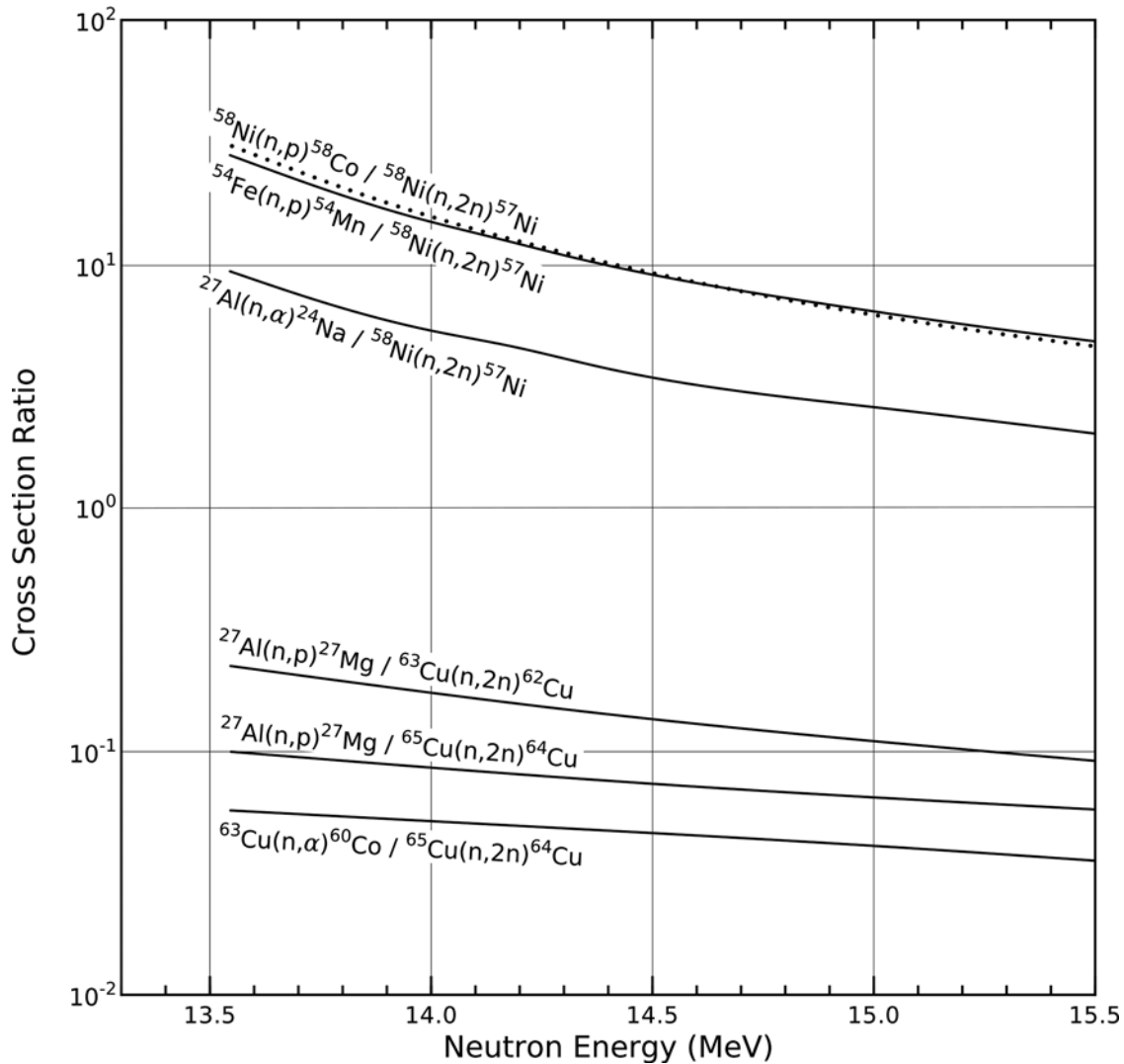
FIG. 7 Ratios of Cross Section for ^3\text{H}(d,n)^4\text{He} Neutron Energy Determination
