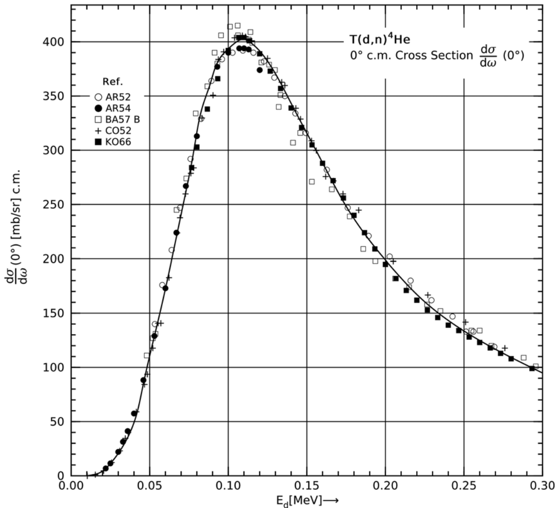
FIG. 2 Variation of 0 Degree {}^3\text{H}(d,n){}^4\text{He} Differential Cross Section with Incident Deuteron Energy (1)
