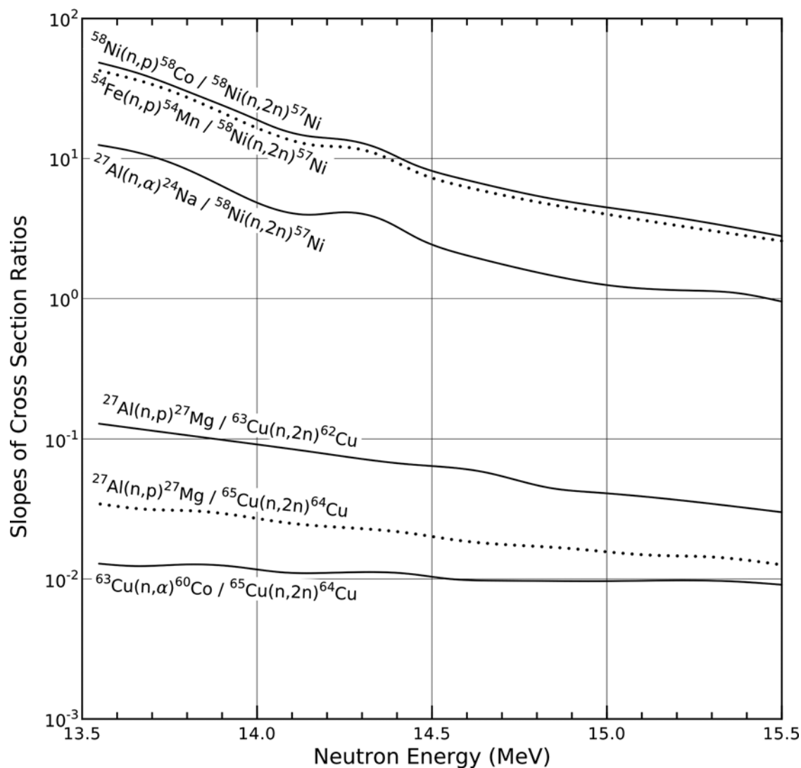
FIG. 8 Slopes of Ratios of Cross Section for ^3\text{H}(d,n)^4\text{He} Neutron Energy Uncertainty Determination
