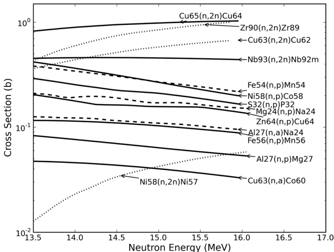
FIG. 6 Cross Sections for Several Reactions Useful for 14-MeV Dosimetry
