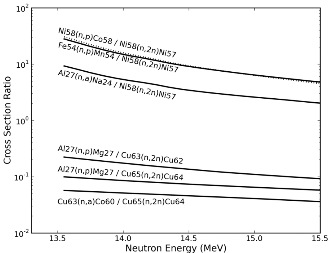
FIG. 7 Ratios of Cross Section for ^3\text{H}(d,n)^4\text{He} Neutron Energy Determination
