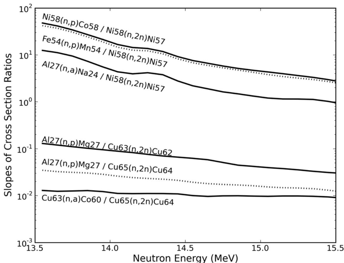
FIG. 8 Slopes of Ratios of Cross Section for ^3\text{H}(d,n)^4\text{He} Neutron Energy Uncertainty Determination
