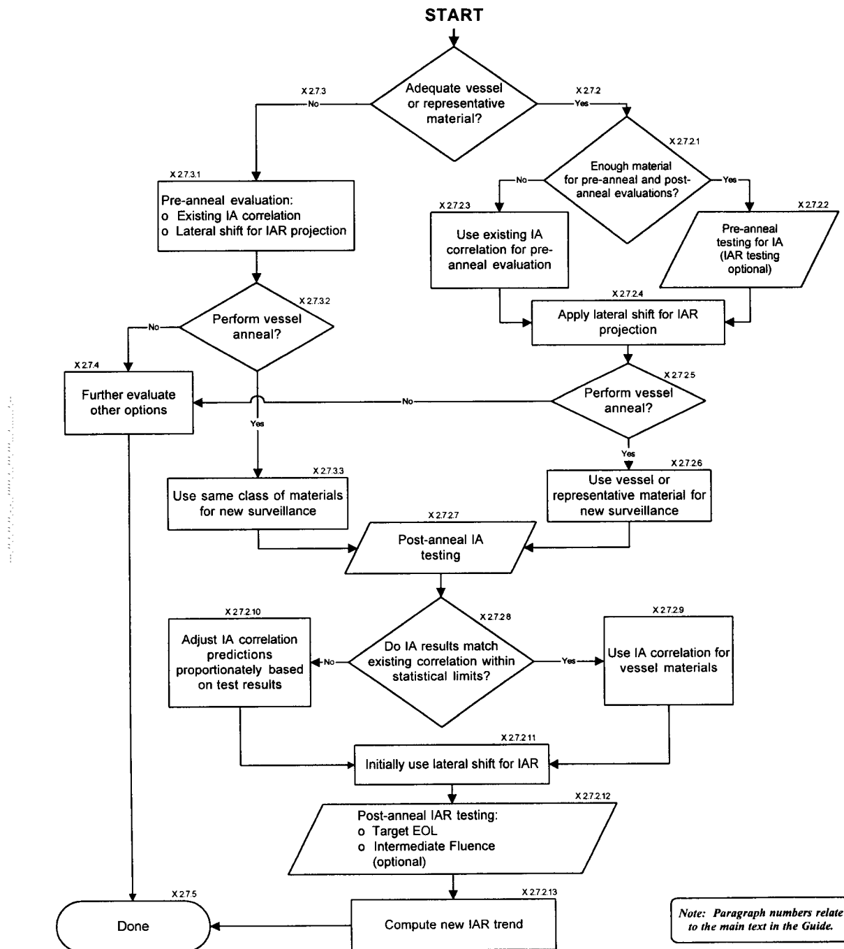
FIG. X2.3 Procedure for Evaluating Annealing Feasibility and Reembrittlement Trend
