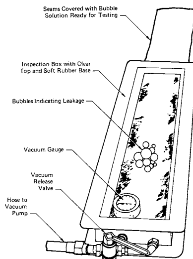
FIG. 2 Vacuum Box
