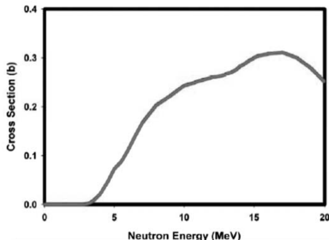
FIG. 1 ^{46}\text{Ti}(n,X)^{46}\text{Sc} Cross Section (Normalized per ^{46}\text{Ti} Atom)
