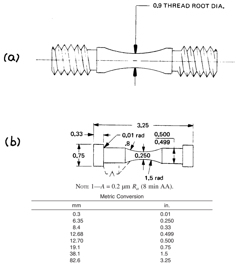
FIG. 1 Standard Hourglass Low Cycle Fatigue Specimen (Threaded Ends (a) and Button Head (b))
