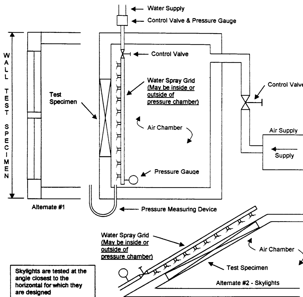
FIG. 1 General Arrangement of the Water Leakage Apparatus Positive Chamber System
