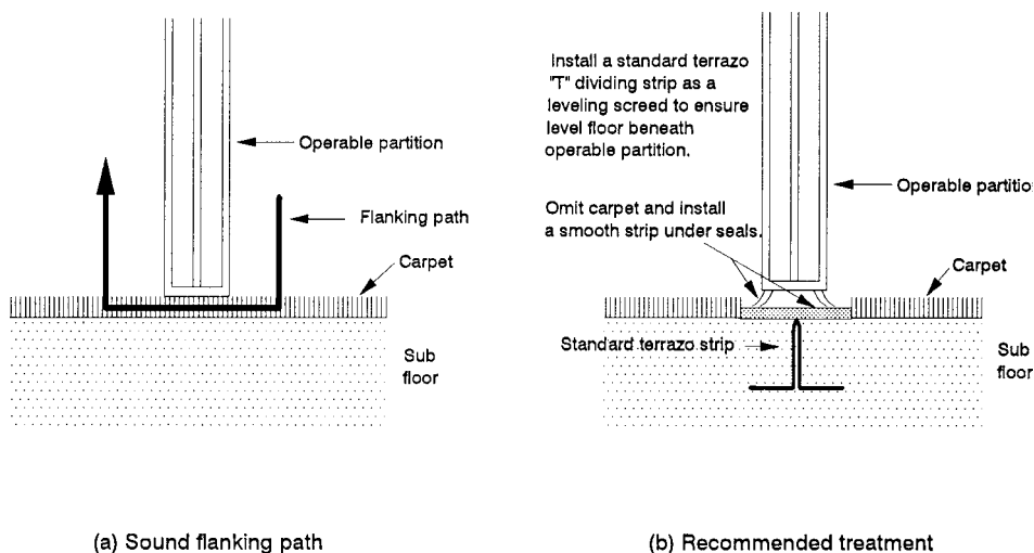
FIG. 5 Recommended Floor Leveling Installation
