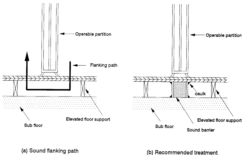
FIG. 4 Recommended Floor Barrier Installation
