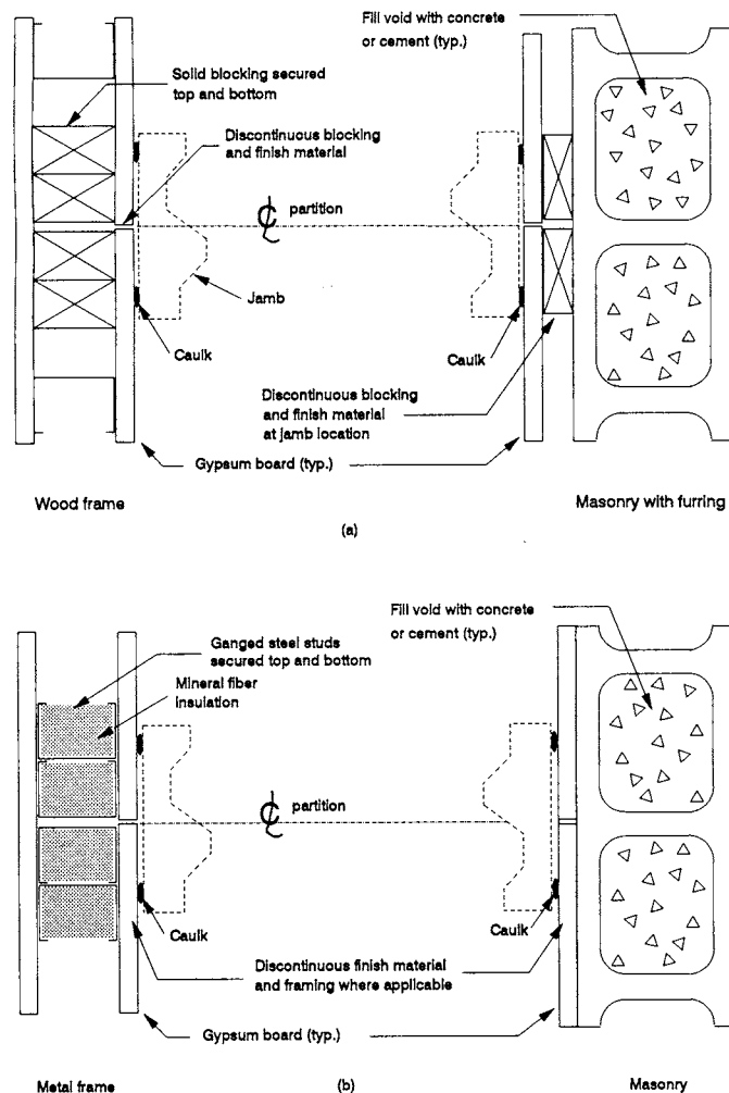
FIG. 6 Typical Wall/Jamb Details
