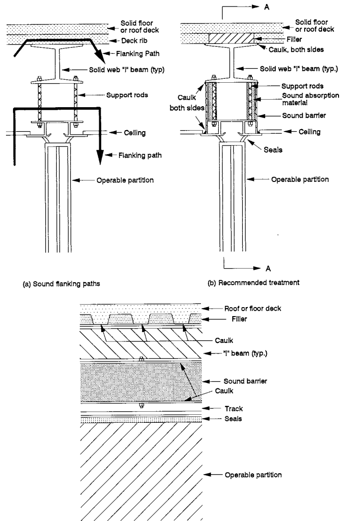
FIG. 1 Recommended Ceiling Barrier Installation
