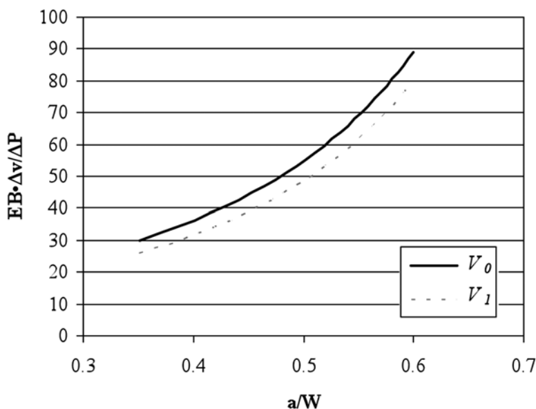
FIG. 12 Compliance Curves for the C(T) Specimen for Two Displacement Measurement Locations V_0 and V_1 shown in Fig. 7
