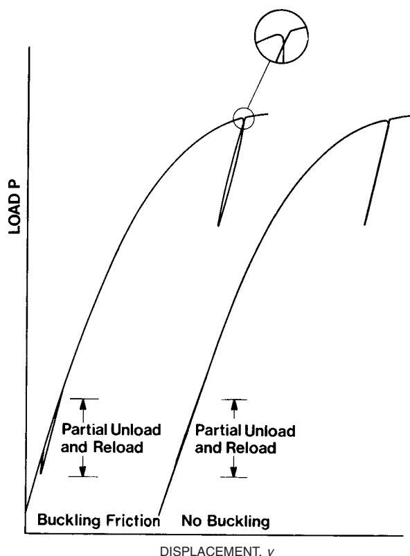
FIG. 9 Detection of Buckling from Compliance Test Records of M(T) and C(T) Specimens
