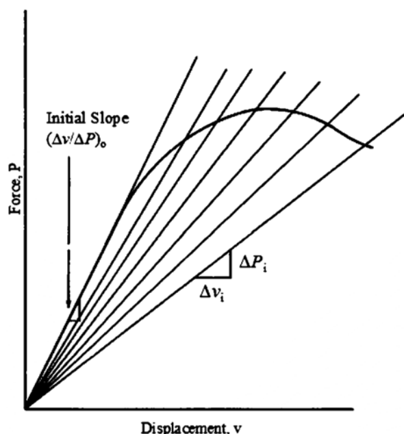
FIG. 10 Schematic Test Record for M(T) or C(T) Specimens
