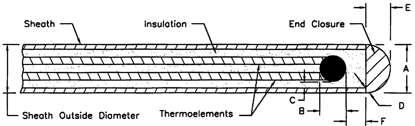
FIG. 1 Grounded Measuring Junction, Style G
