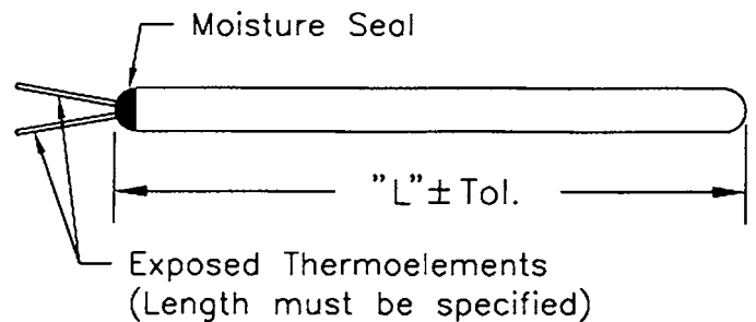
FIG. 4 Sheathed Thermocouple with Exposed Wires
