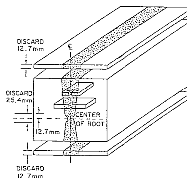
FIG. 1 Specimen Orientation and Location in Plate, Forging, and Weld Deposit Materials: A) Crack Plane Orientation Code; B) Plate and Forging Specimen Location and Orientation; C) Weld Specimen Location and Orientation
