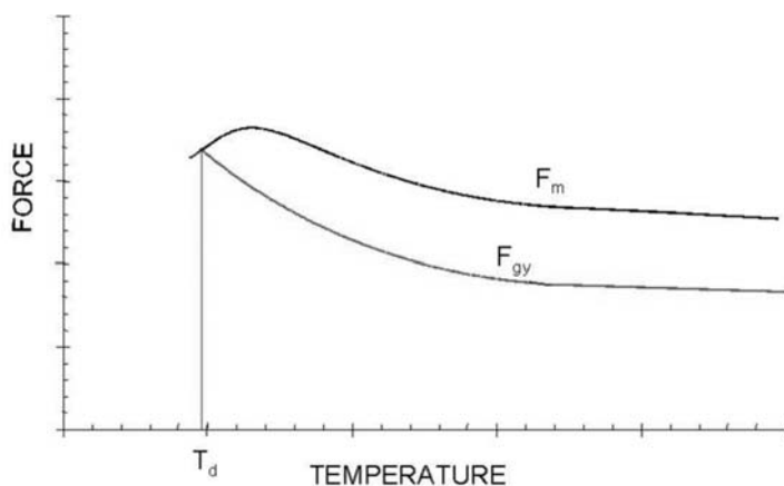
FIG. 5 Effects of Temperature on F_{gy} and F_m
