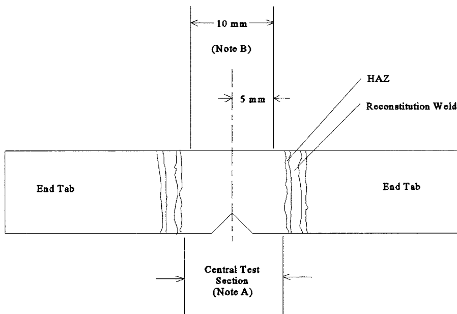
FIG. 2 Example of Reconstituted Charpy-type Specimen
