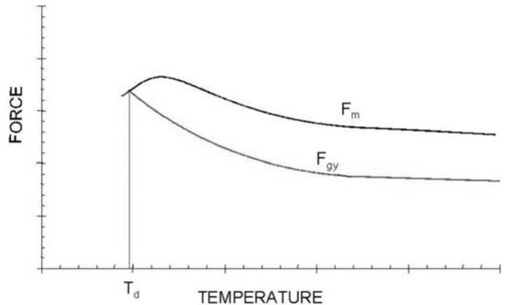
FIG. 5 Effects of Temperature on F_{gy} and F_m
