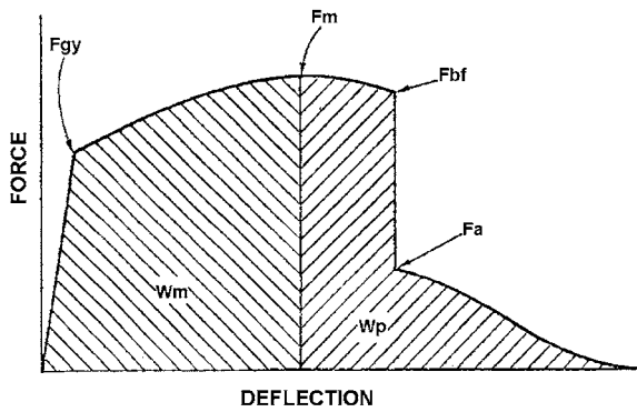
FIG. 4 Idealized Force Deflection Record
