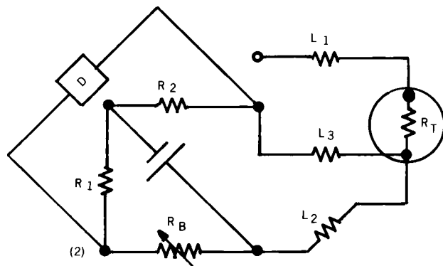
FIG. X1.2 Two Measurement Method for Determining the Resistance of a Three-Wire Thermometer Employing a Simple Bridge
