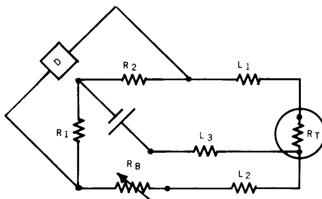
FIG. X2.2 Determination of the Resistance of a Three-Wire Thermometer Employing a Modified Bridge
