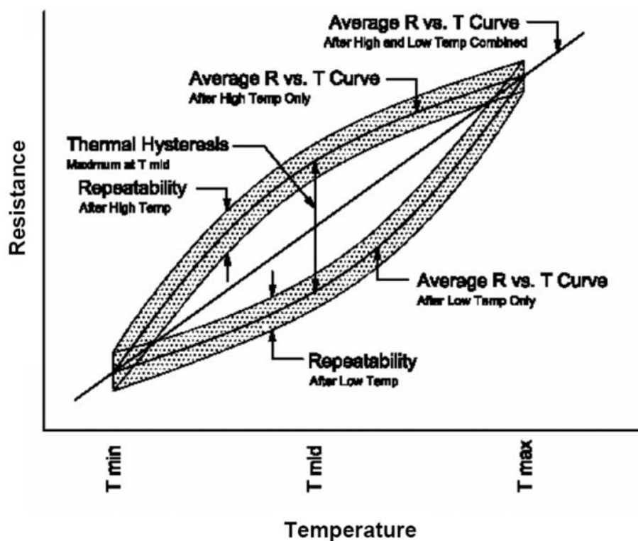
FIG. 5 Exaggerated representation of Thermal Cycle Repeatability and Thermal Hysteresis
