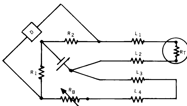
FIG. X2.3 Determination of the Resistance of a Compensated Four-Wire Thermometer Employing a Modified Bridge
