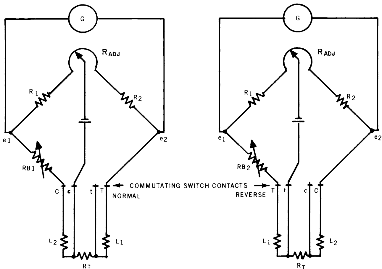
NOTE 1—Assumes that L_1 = L_2 or that the difference (L_1 - L_2) is constant over the period of measurement. FIG. X2.4 Determination of the Resistance of a Four-Terminal Thermometer Employing a Mueller Bridge
