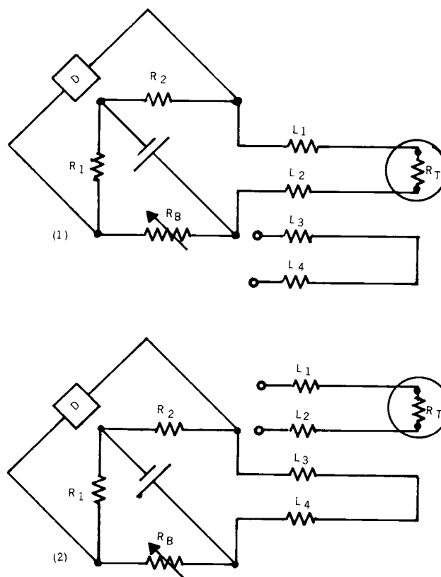
FIG. X1.3 Two-Measurement Method for Determining the Resistance of a Compensating Loop Four-Wire Thermometer Employing a Simple Bridge
