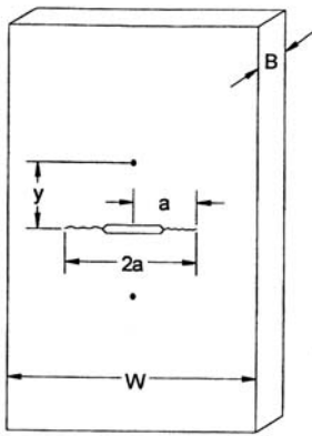
Middle-Tension, M(T) Specimen
