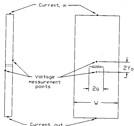
FIG. A2.4 M(T) Geometry and Electric Potential Wire Displacement Locations for Eq A2.5 (41)
