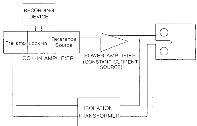
FIG. A6.2 Schematic Diagram of the AC Potential System (60)
