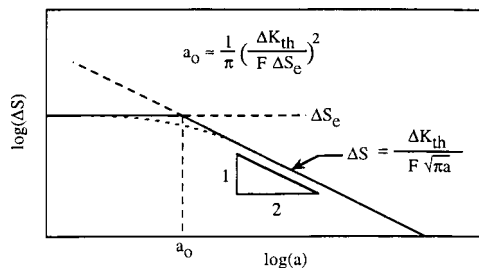
FIG. X3.1 Diagram for Estimating a_0
