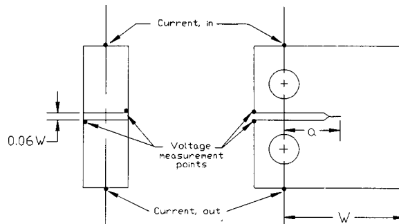
FIG. A1.5 C(T) Geometry and Electric Potential Wire Placement Locations for Eq A1.4 (68)
