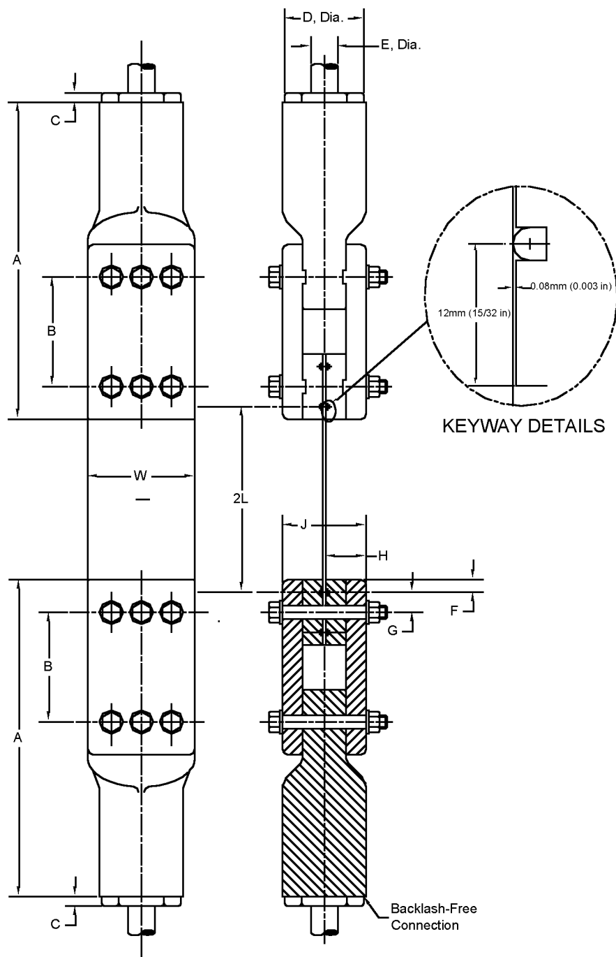
FIG. A2.2 Example of Bolt and Keyway Assembly for Gripping 100-mm (4-in.) wide M(T) Specimen
