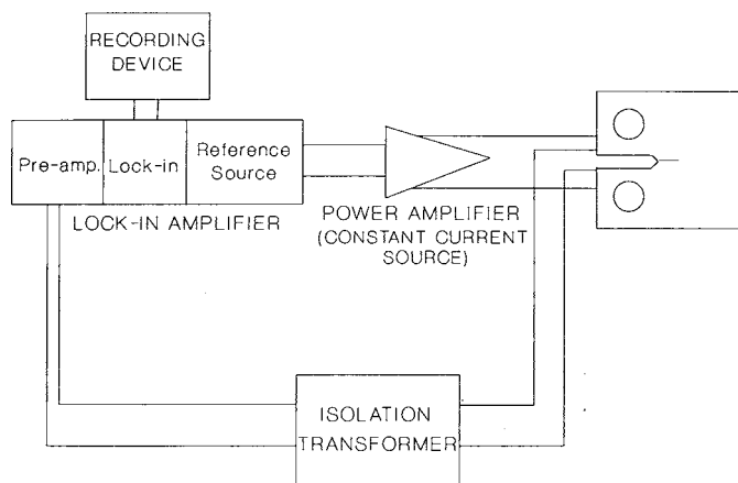
FIG. A6.2 Schematic Diagram of the AC Potential System (60)
