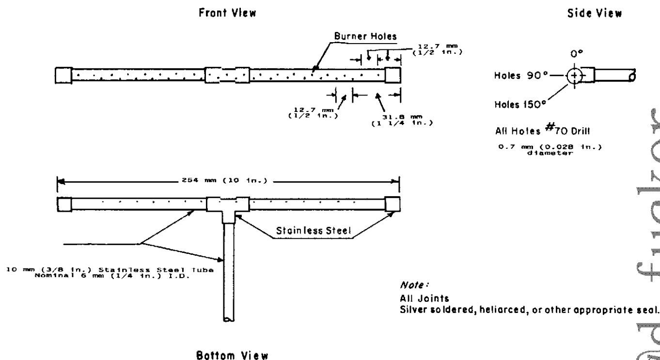
FIG. 5 Pilot Burner
