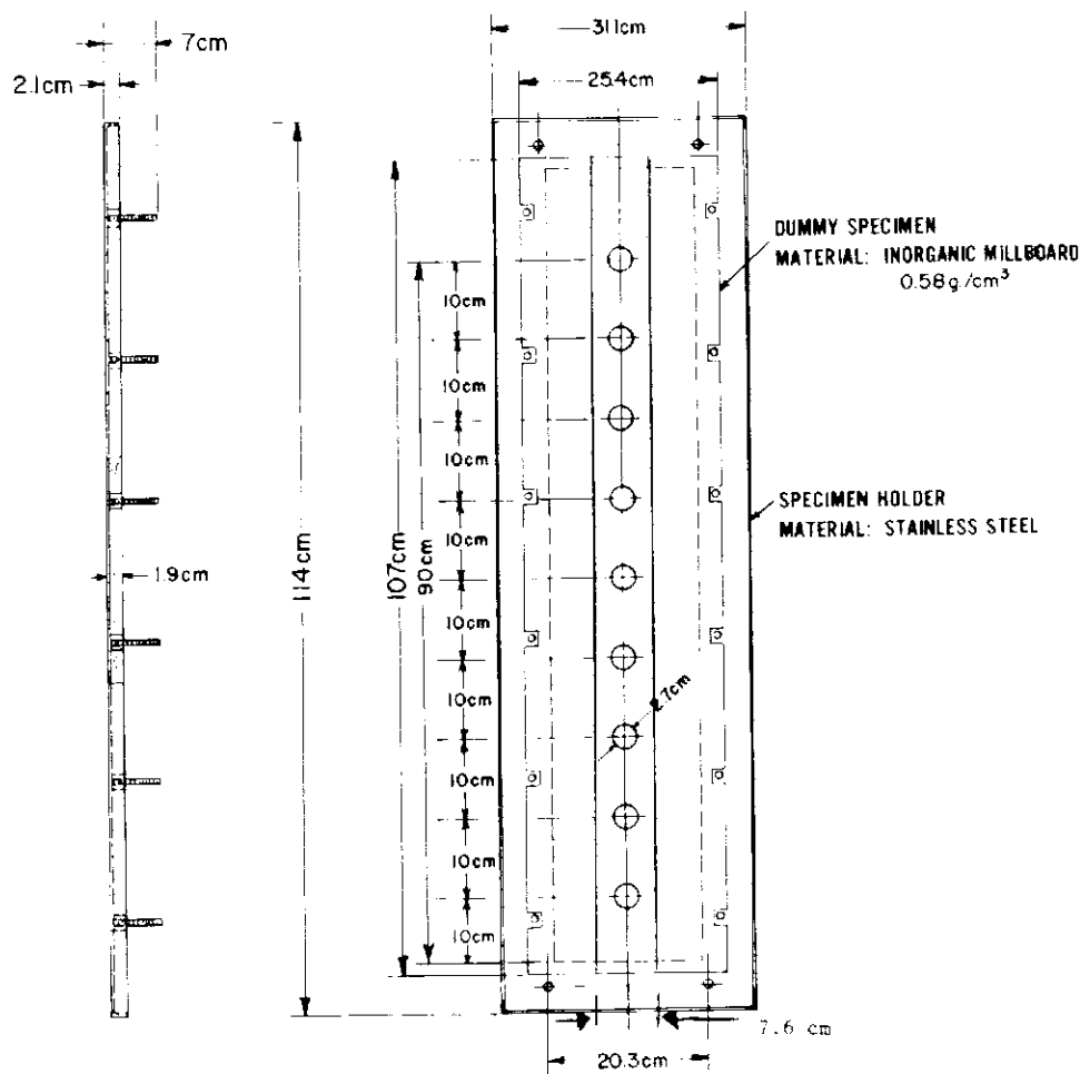
FIG. 6 Dummy Specimen in Specimen Holder
