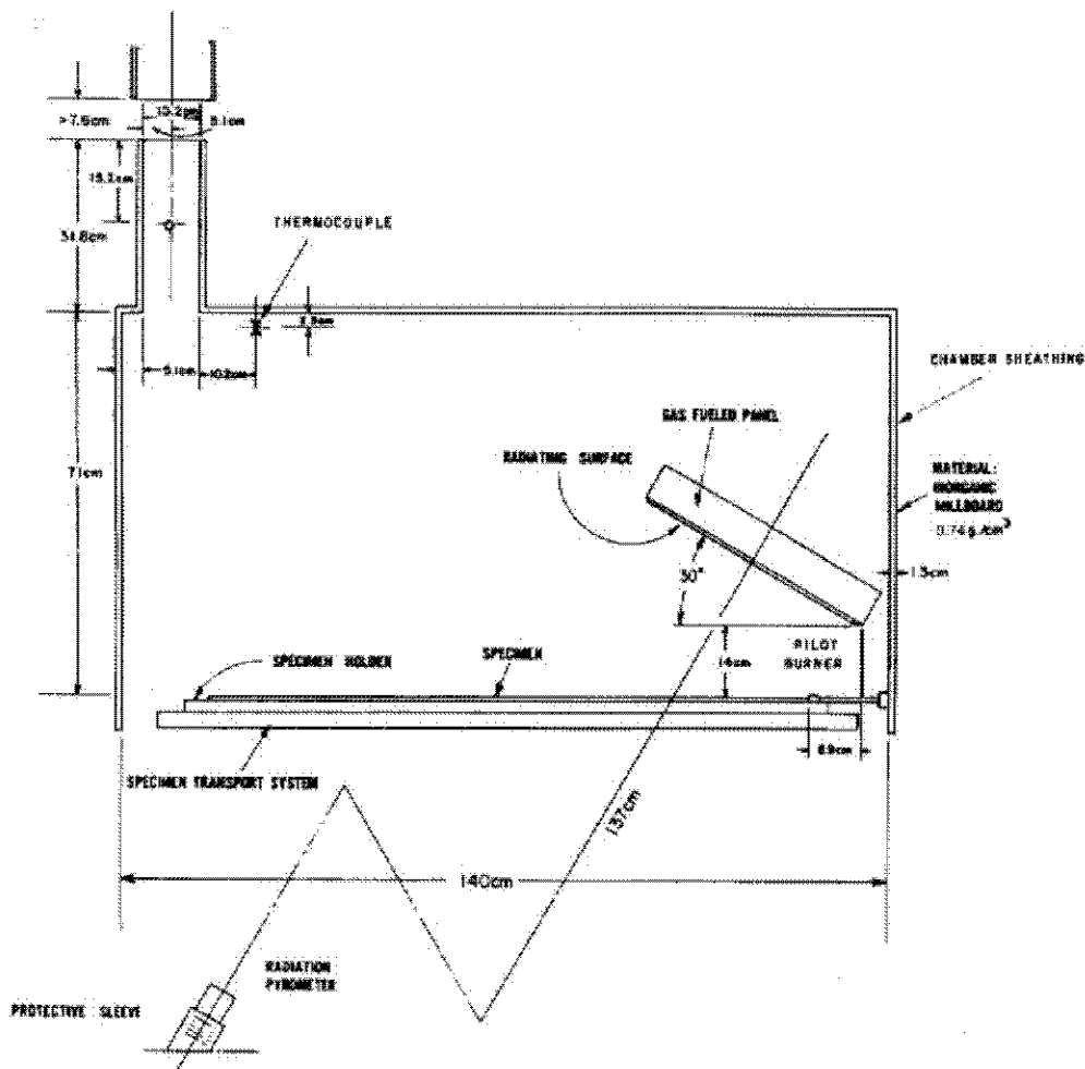
FIG. 3 Flooring Radiant Panel Tester Schematic Side Elevation
