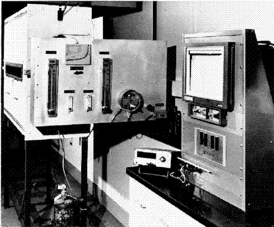
FIG. X3.1 Historic Photograph of Flooring Radiant Panel Tester Apparatus
