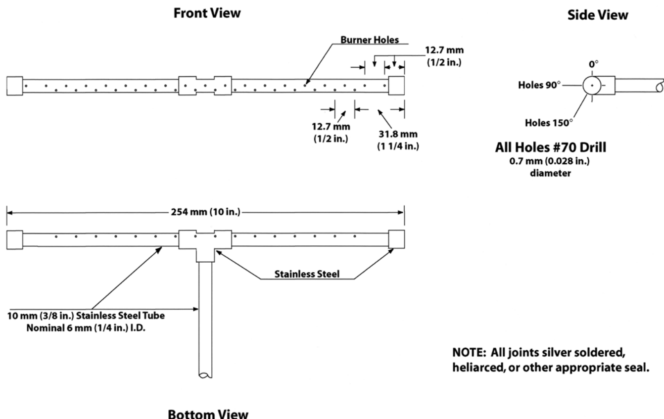
FIG. 6 Pilot Burner
