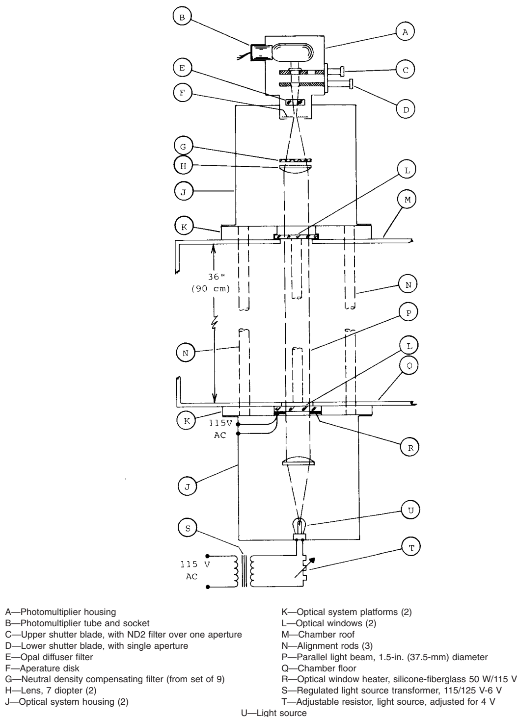
FIG. 5 Photometer Details
