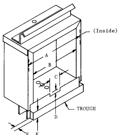
SAMPLE HOLDER
