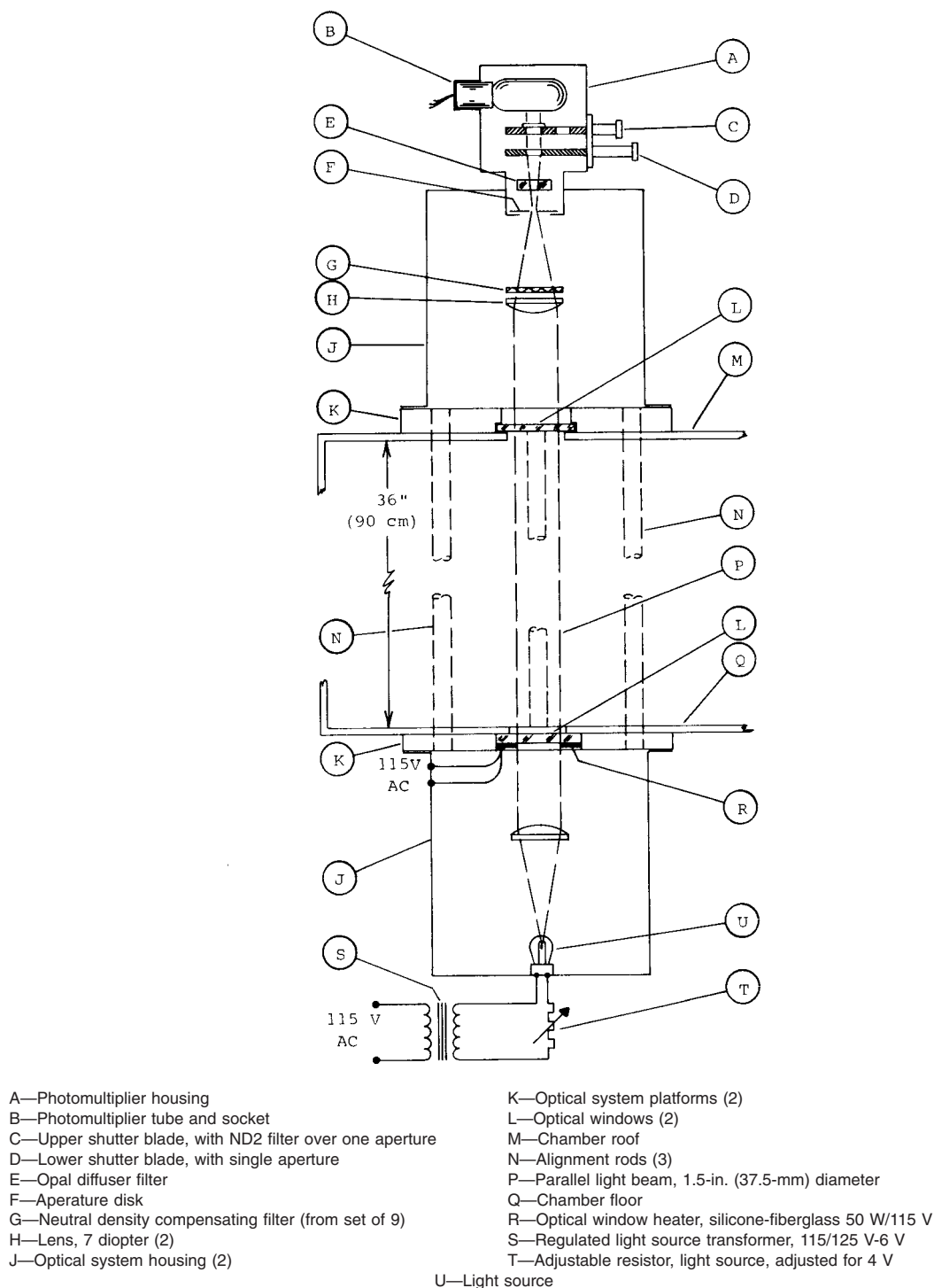
FIG. 5 Photometer Details
