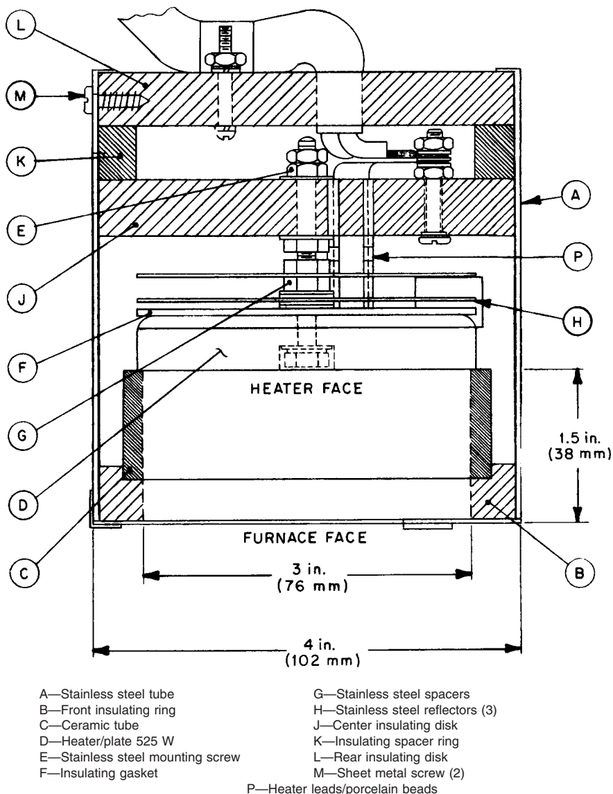
FIG. 2 Furnace Section
