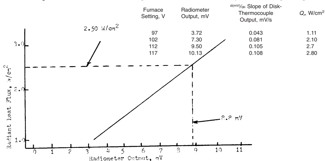
FIG. A1.2 Example—Calibration of Radiometer
