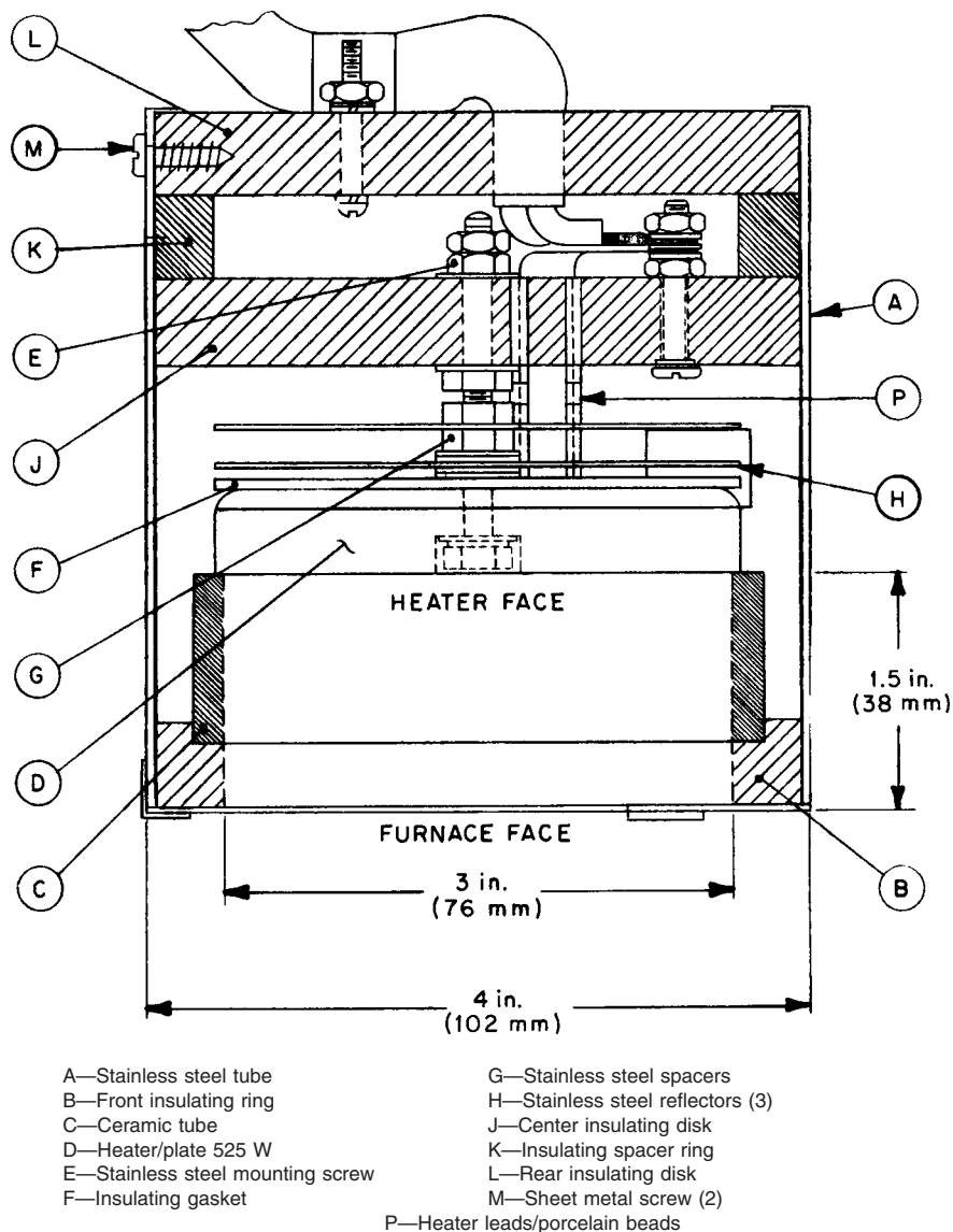
FIG. 2 Furnace Section
