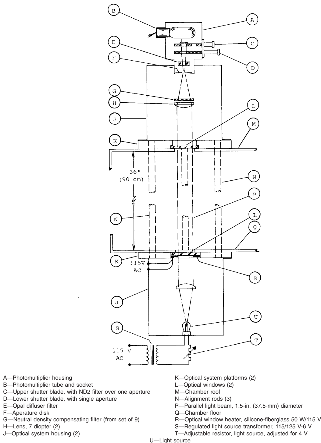
FIG. 5 Photometer Details
