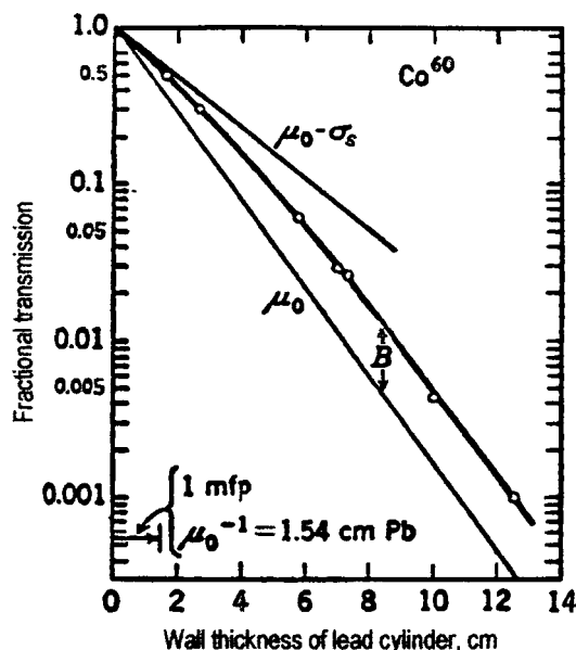
FIG. X5.1 Transmission of ^{60}\text{Co} \gamma rays through cylindrical lead shields. Theoretical lines for the transmission of primary photons ( \mu_0 ) and for the true absorption of primary energy ( \mu_0 - \sigma_s ) are shown for comparison. [Figure from Evans (5).]
