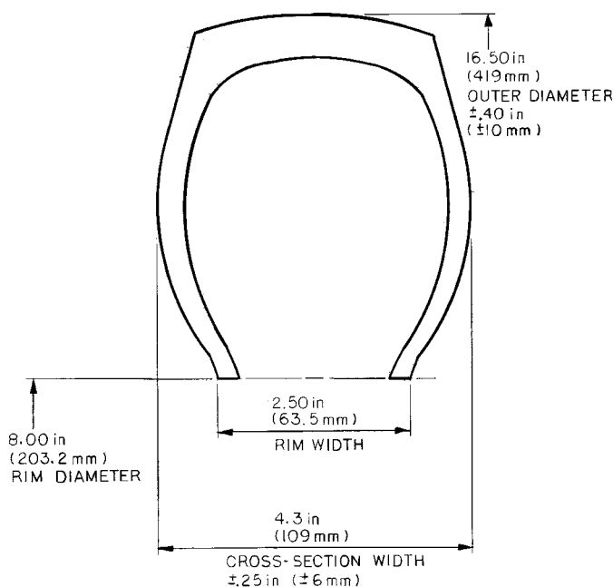
FIG. A2.2 Alternate Mu-Meter Tire Dimensions
