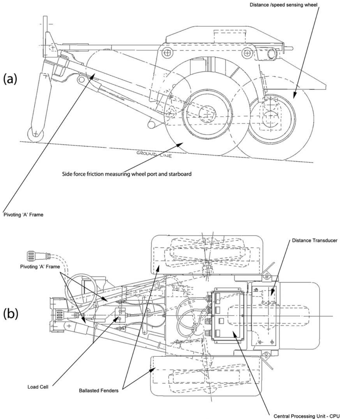
FIG. 1 Mu-Meter Schematics
