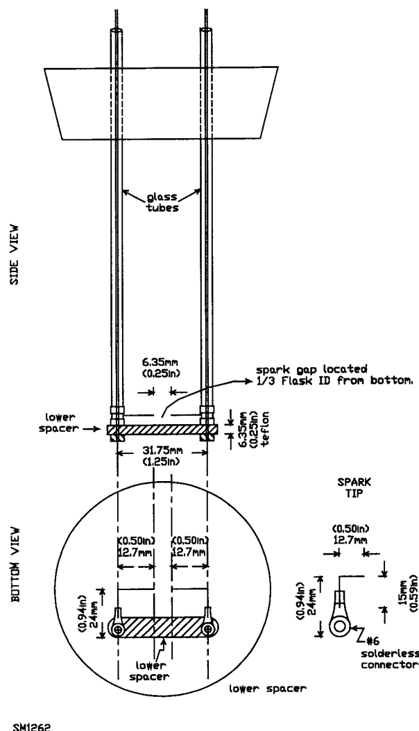
FIG. A1.2 Spark Electrode Set-up
