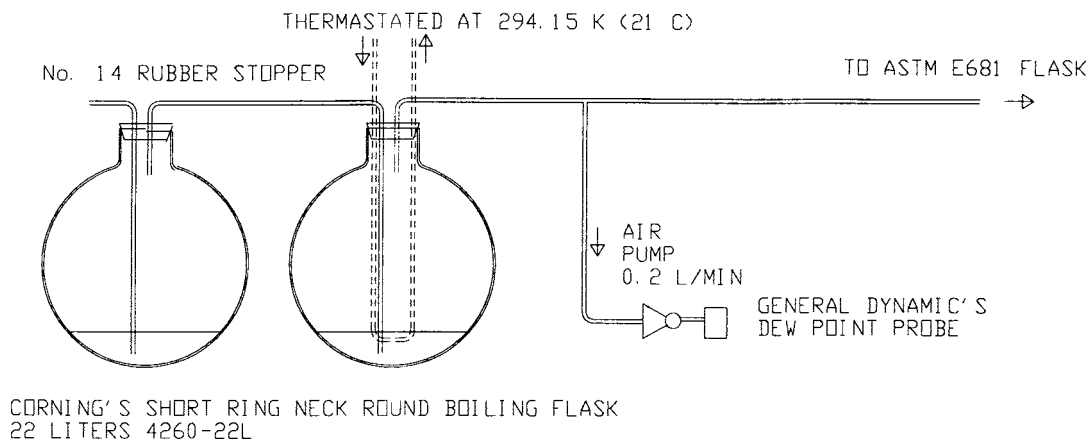
FIG. A1.3 Air Humidifier Set-up
