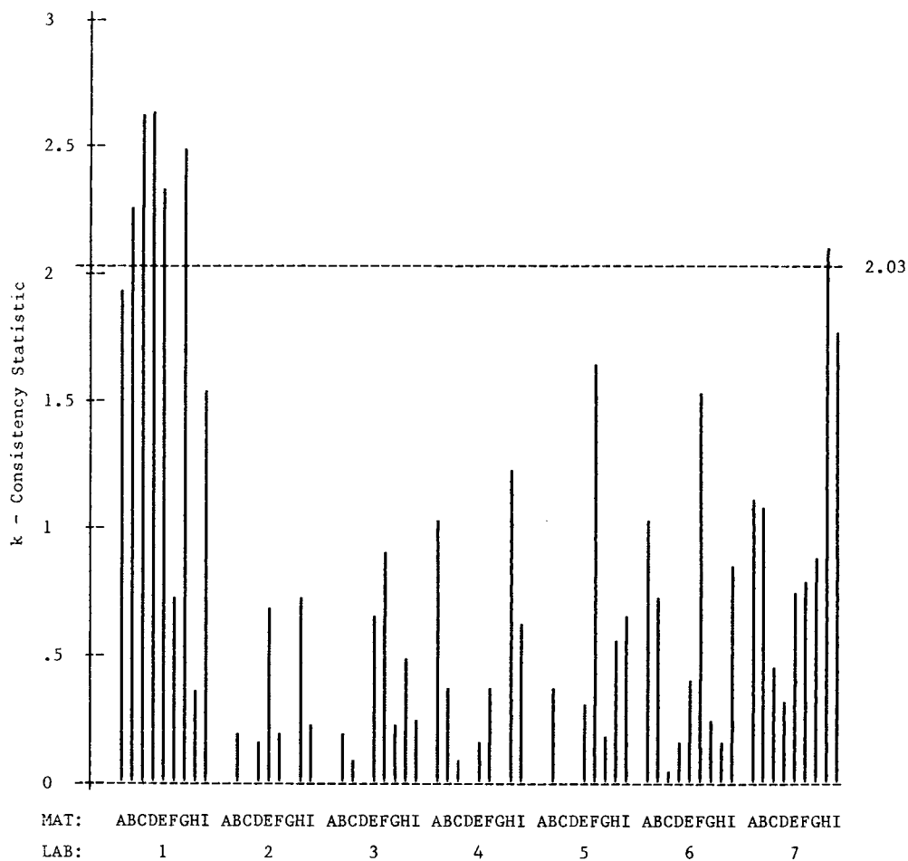
FIG. 5 Pentosans in Pulp: k —Materials within Laboratories
