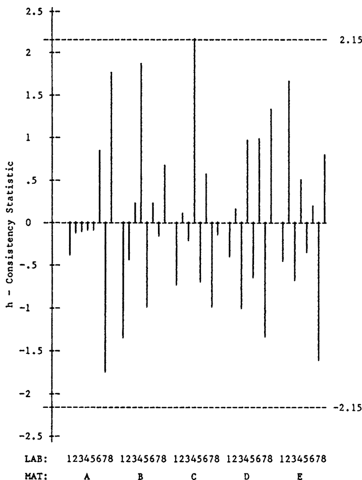
FIG. 3 Glucose in Serum: h —Laboratories within Materials
