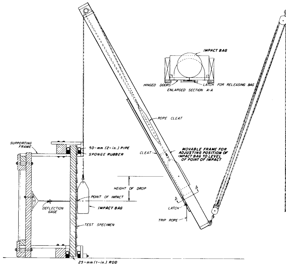
FIG. 3 Impact Load Test (Specimen Vertical)
