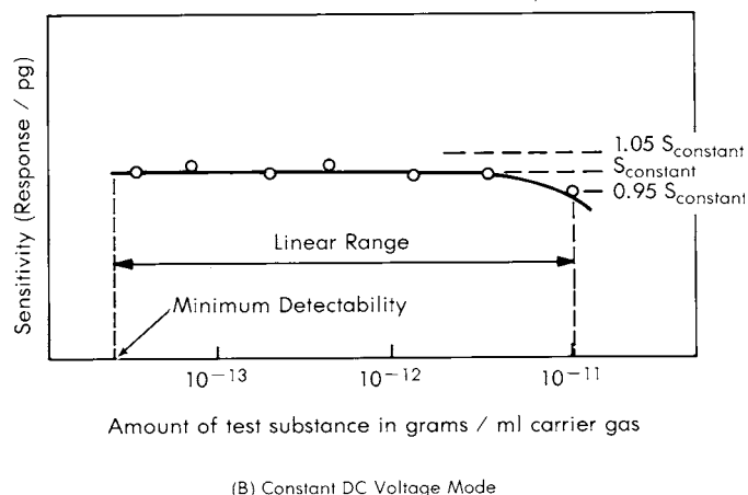
FIG. 1 Example of a Linearity Plot for an Electron-Capture Detector
