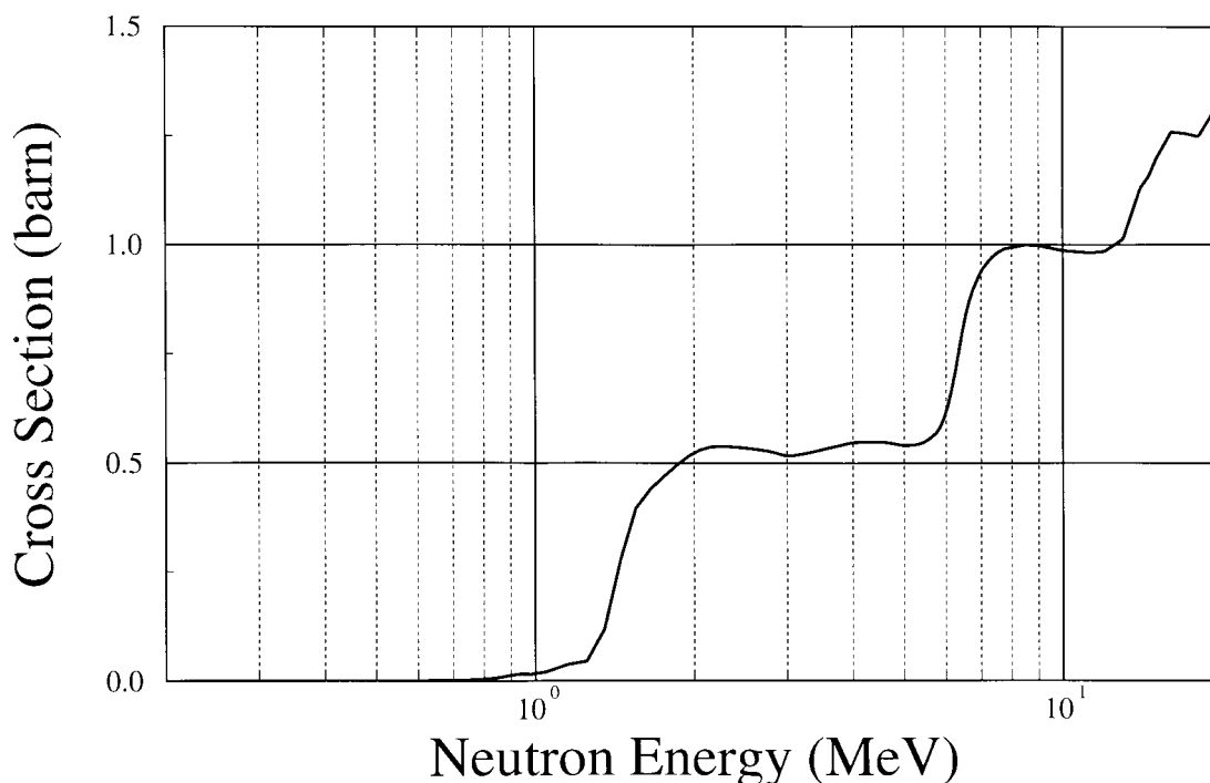
FIG. 1 ENDF/B-VI Cross Section Versus Energy for the ^{238}\text{U}(\text{n},\text{f})\text{F.P.} Reaction
