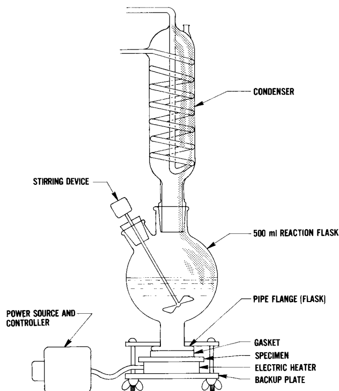
FIG. 1 Schematic of Apparatus for Heat-Rejecting Surface Test
