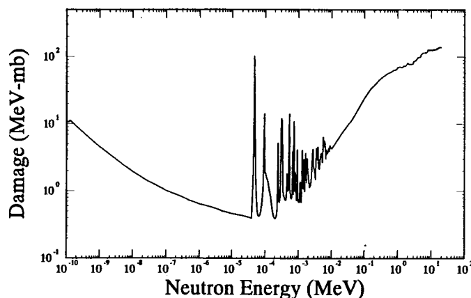
FIG. A2.3 GaAs Damage Function
