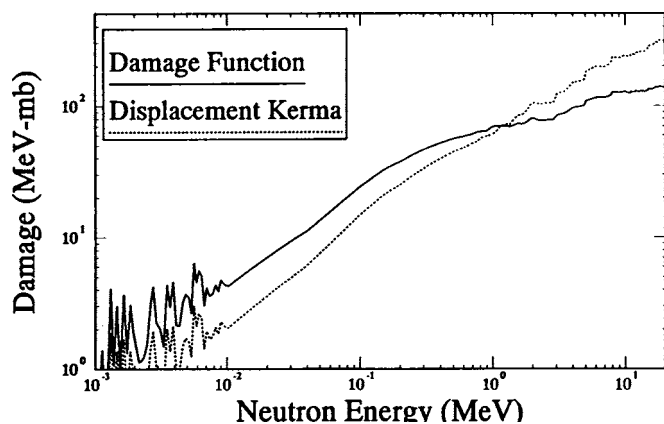
FIG. A2.2 Comparison of GaAs Microscopic Displacement Kerma and Damage Function
