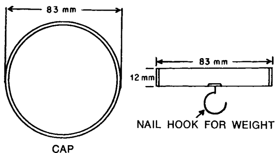
FIG. 1 Typical Cohesion/Adhesion Testing Apparatus
