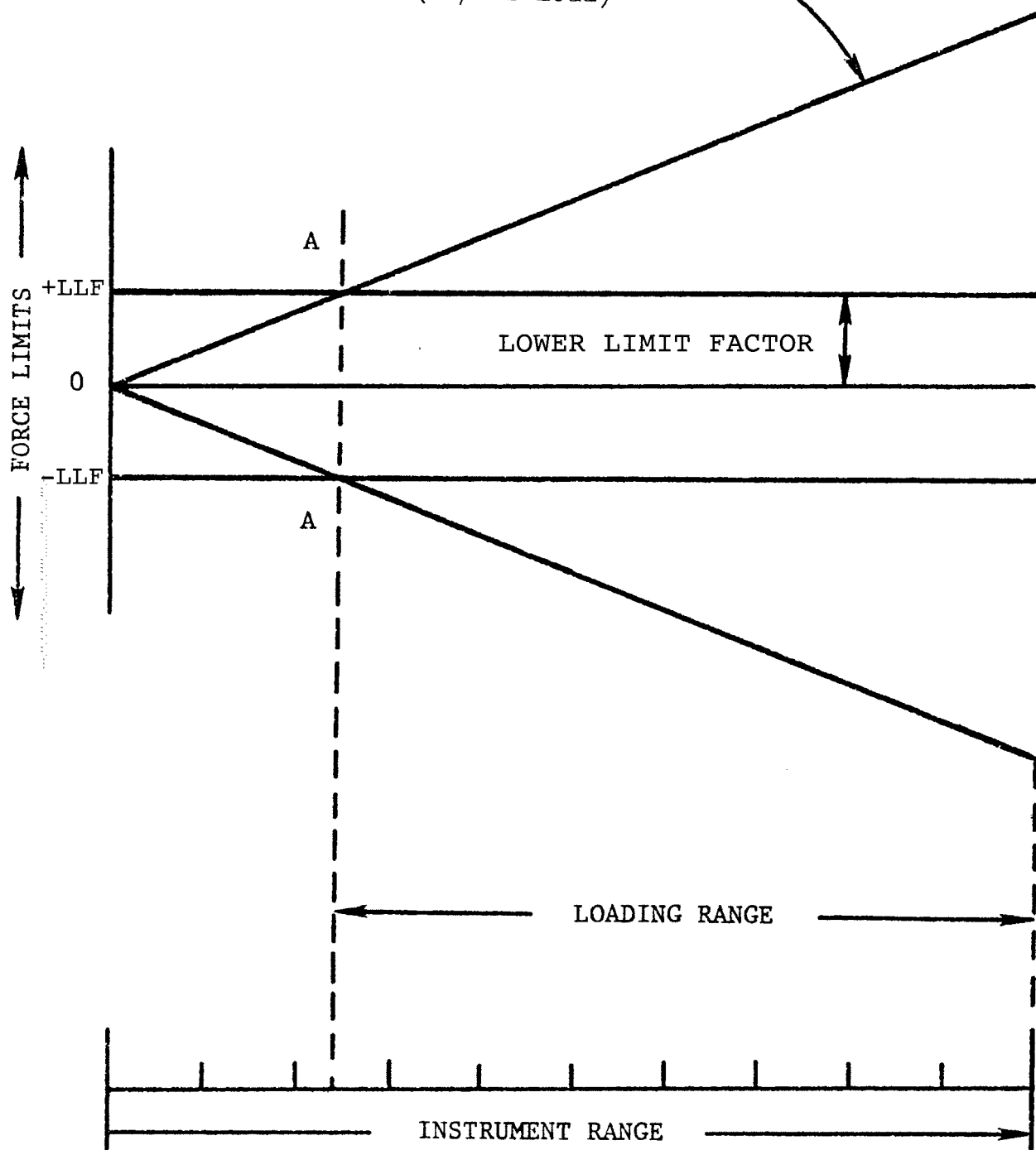
FIG. 1 Relationship of Loading Range to Instrument Lower Force Limit and Specified Limits of Error
