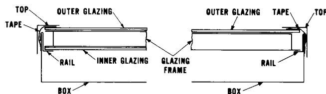
FIG. 5 Natural Weathering Box Assembly—Rigid Glazing
