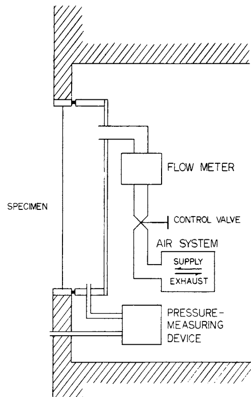
FIG. 1 General Arrangement of Air Leakage Test Apparatus
