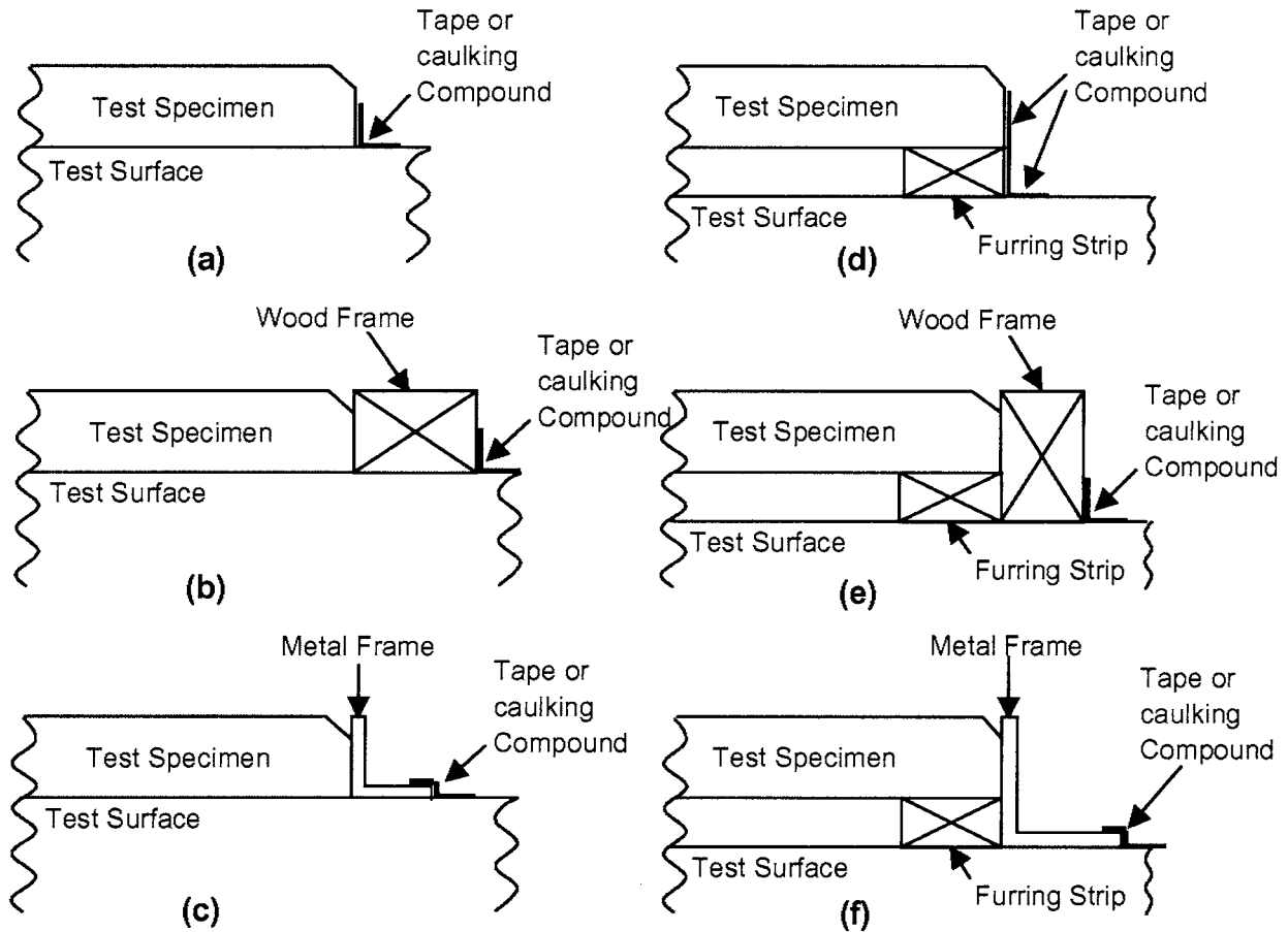
FIG. 1 Type A Mounting
