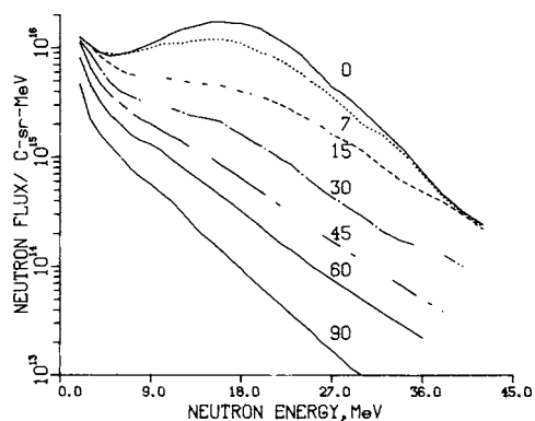
FIG. 1 Flux Contours for RTNS II
