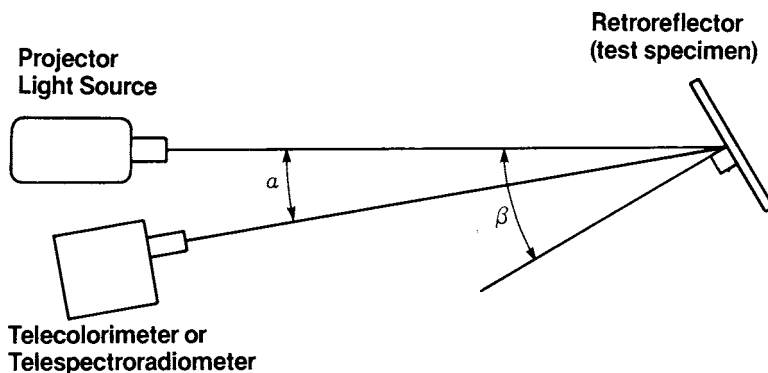
FIG. 1 Simplified Geometric Arrangement of Apparatus for Measurement of Chromaticity of Test Specimen
