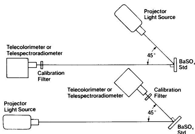
FIG. 2 Two Arrangements Suitable for Calibration of Telecolorimeter or Telespectroradiometer
