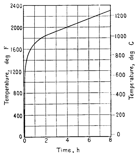
FIG. 1 Temperature-Time Curve
