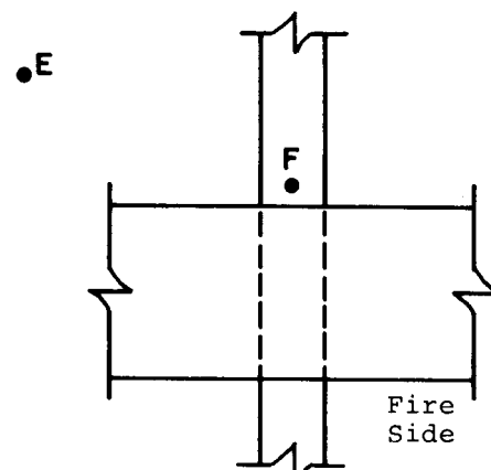
Floor Assembly-Elevation View Wall Assembly-Plan View
