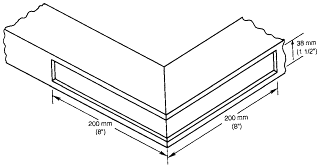
FIG. 3 Slots for Corner Straps of Cover Holder
