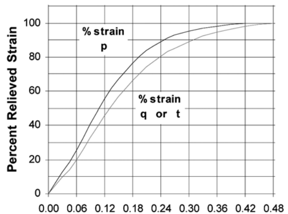
FIG. 6 Typical Plots of Percent of Strain versus Depth for Uniform Through-Thickness Stress, (a) Rosette Types A & B, (b) Rosette Type C
