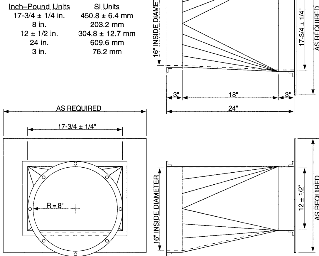
FIG. 3 Typical Exhaust End Transition (Not a Construction Drawing)
