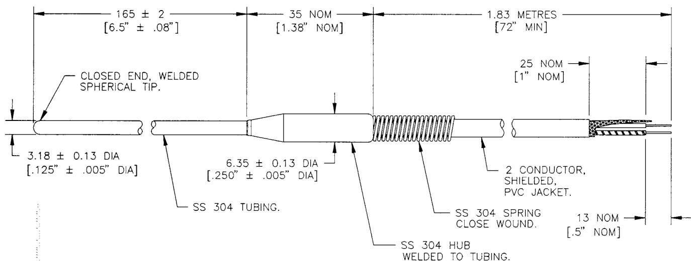
FIG. 5 General Purpose Two-Wire Sensor in Stainless Steel Housing
