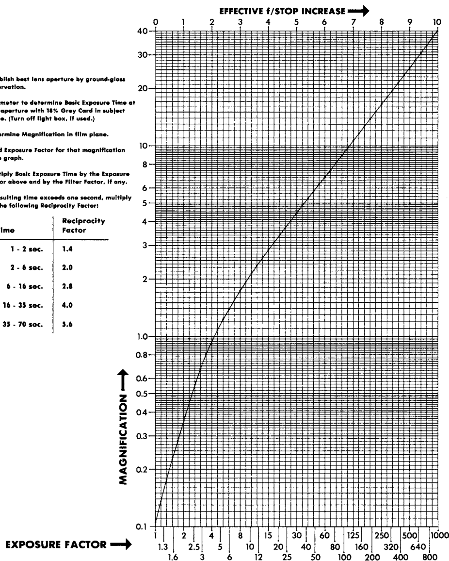
FIG. X2.1 Photomacrography Exposure Computer
