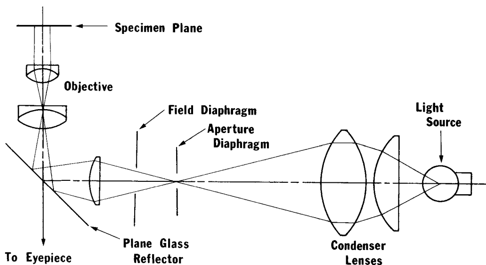
FIG. 1 Vertical Illuminating System for a Metallurgical Microscope
