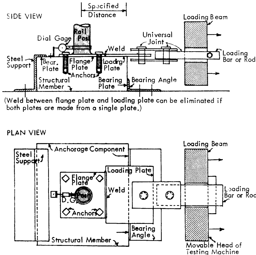
FIG. 3 Diagrammatic Test Set-up for Applying Shear Force to Rail Flange, Rail-Post Flange, and Flange Anchors
