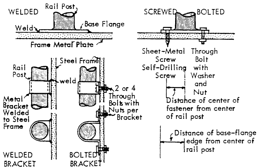
NOTE—Brackets are also used for fastening to other materials with appropriate anchors. FIG. X1.3 Typical Ways of Anchoring Metal Railings and Rails to Steel Framing
